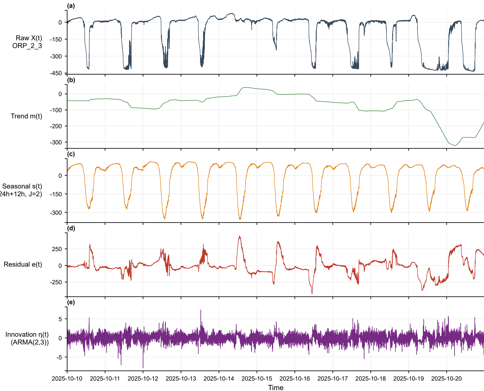
Multi-scale decomposition — ORP_2_3 (pre_anoxic_rear, min) [2025-10-10~2025-10-20]
